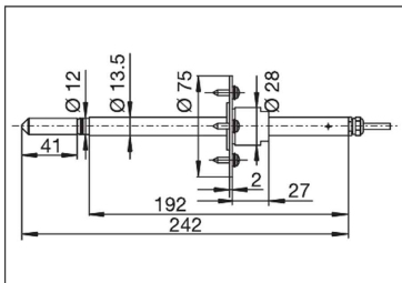
Probe, type 907023/335 (mounting flange is optional)
