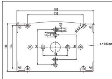
Plastic mounting plate or drilling template
