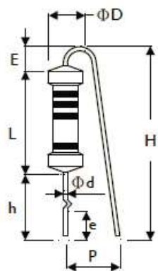
FK TYPE
