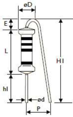
F TYPE
